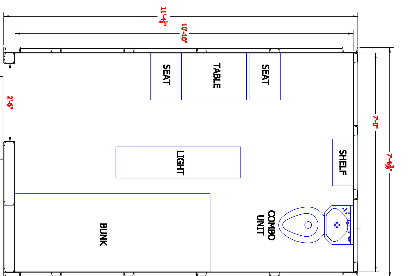
TYPE "1H" REAR CHASE CELL ENGINEERED AREA: 24.63 SQ. FT. UNENGINEERED AREA: 52.1 SQ. FT. TOTAL AREA: 76.73 SQ. FT.
