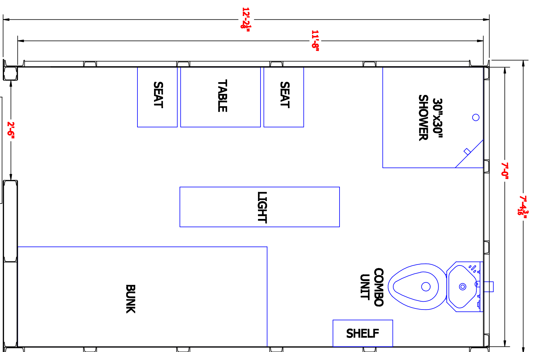
TYPE "2H" REAR CHASE CELL ENGINEERED AREA: 31.2 SQ. FT. UNENGINEERED AREA: 31.4 SQ. FT. TOTAL AREA: 62.6 SQ. FT.
