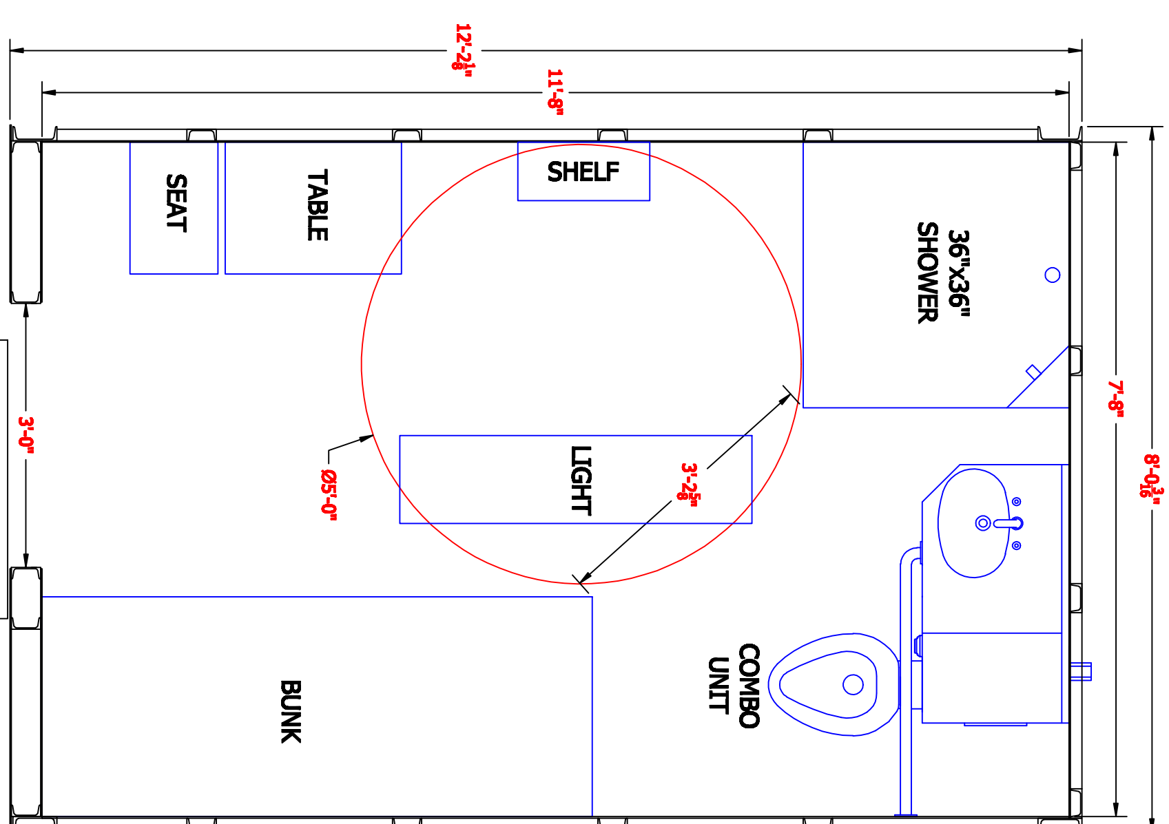
TYPE "2H" REAR CHASE H.C. CELL ENGINEERED AREA: 35.8 SQ. FT. UNENGINEERED AREA: 54.7 SQ. FT. TOTAL AREA: 90.5 SQ. FT.
